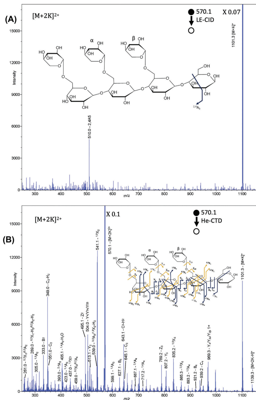
FIGURE 4 Product ion mass spectra of XXXG with insets of the product ion map for each activation technique: (A) low-energy collision-induced dissociation (LE-CID) of [M + 2K]^{2+} precursor at m/z 570.1 with an excitation amplitude of 0.8 arbitrary units, a low-mass cutoff (LMCO) of m/z 250, and a precursor isolation width of 4 Da and (B) He-CTD of [M + 2K]^{2+} precursor at m/z 570.1 with an identical LMCO and precursor isolation width as the LE-CID spectrum. Dark blue arrows represent unambiguous product ion identities, and gold arrows represent ambiguous product ion identities due to alternative isobaric product ions. Bold labels in the product ion map represent singly charged product ions, and nonbolded labels are doubly charged product ions
