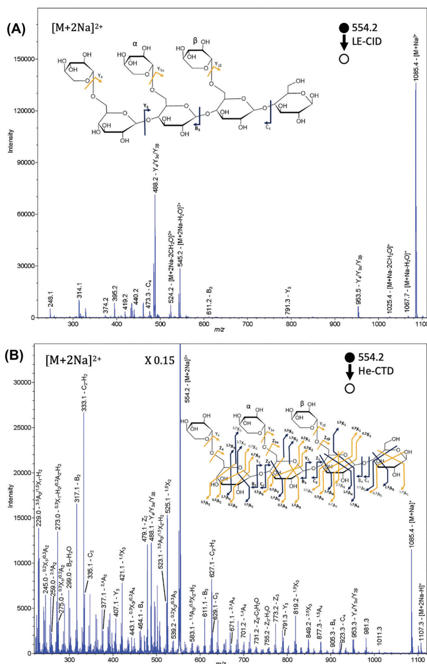
FIGURE 1 Product ion mass spectra of XXXG with insets of the product ion map for each activation technique: (A) low-energy collision-induced dissociation (LE-CID) of [\text{M} + 2\text{Na}]^{2+} precursor at m/z 554.2 with an excitation amplitude of 0.8 arbitrary units, a low-mass cutoff (LMCO) of m/z 220, and a precursor isolation with of 4 Da and (B) helium charge transfer dissociation (He-CTD) of [\text{M} + 2\text{Na}]^{2+} precursor at m/z 554.2 with an identical LMCO and isolation width as the LE-CID spectrum. Dark blue arrows represent unambiguous identities; gold arrows represent ambiguous identities caused by alternative isobaric product ions. Bold labels in the product ion map represent singly charged product ions, and nonbold labels are doubly charged product ions
