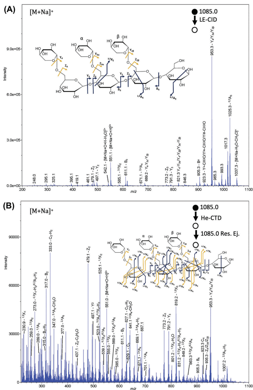
FIGURE 2 Product ion mass spectra of XXXG with insets of the product ion map for each activation technique: (A) low-energy collision-induced dissociation (LE-CID) of [M + \text{Na}]^+ precursor at m/z 1085.0 with an excitation amplitude of 0.8 arbitrary units, a low-mass cutoff (LMCO) of m/z 220, and a precursor isolation width of 3 Da and (B) helium charge transfer dissociation (He-CTD) of [M + \text{Na}]^+ precursor at m/z 1085.0 with a 5-V resonance ejection of unreacted precursor ions at m/z 1085.0 between CTD activation and mass acquisition and an identical LMCO and isolation width as the LE-CID spectrum. Dark blue arrows represent unambiguous identities; gold arrows represent ambiguous identities caused by alternative isobaric product ions. Bold labels in the product ion map represent singly charged product ions, and nonbold labels are doubly charged product ions
