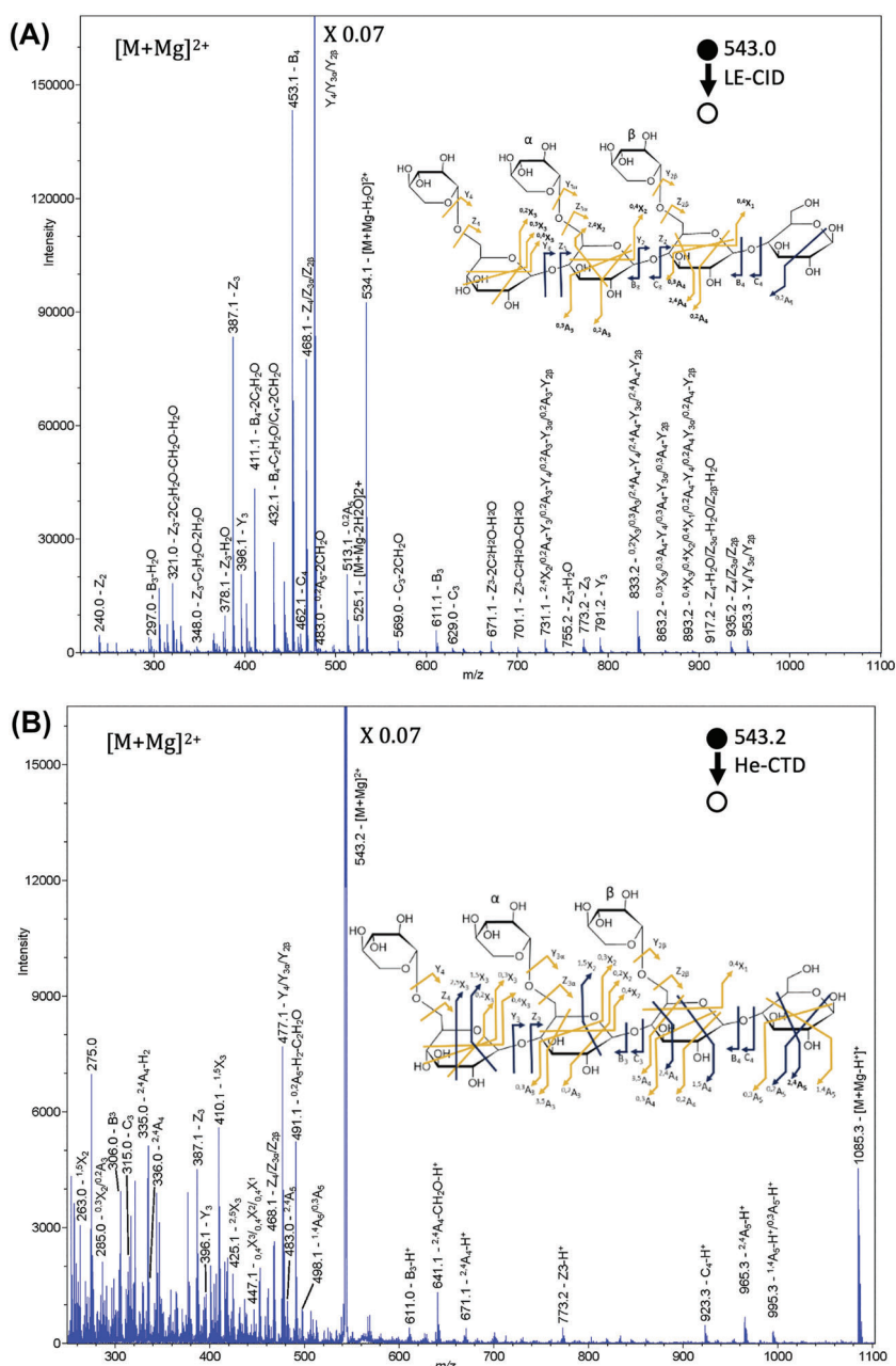
FIGURE 5 Product ion mass spectra of XXXG with insets of the product ion map for each activation technique: (A) low-energy collision-induced dissociation (LE-CID) of [M + Mg]^{2+} precursor at m/z 543.0 with an excitation amplitude of 0.8 arbitrary units, a low-mass cutoff (LMCO) of m/z 250, and a precursor isolation width of 4 Da and (B) helium charge transfer dissociation (He-CTD) of [M + Mg]^{2+} precursor at m/z 543.2 with an identical LMCO and precursor isolation width as the LE-CID spectrum. Dark blue arrows represent unambiguous product ion identities, and gold arrows represent ambiguous product ion identities due to alternative isobaric product ions. Bold labels in the product ion map represent singly charged product ions, and nonbolded labels are doubly charged product ions
